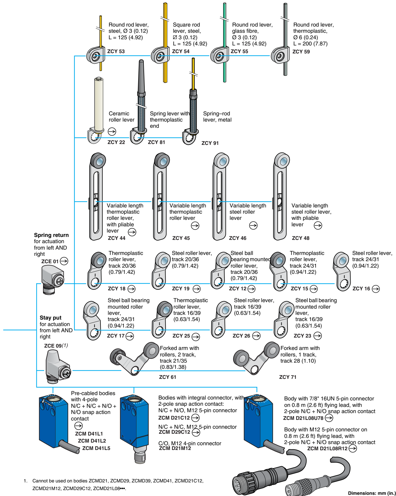
Dimensions: mm (in.)
